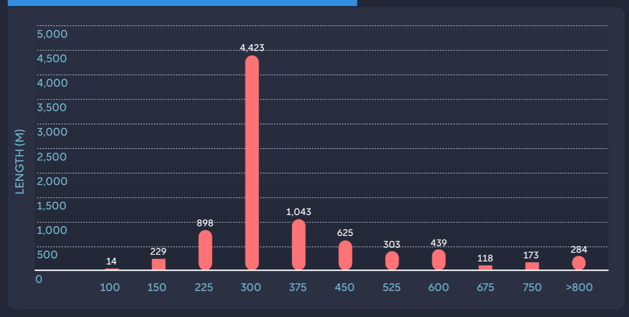
FIGURE 3 Distribution of Stormwater Pipe Assets by Size
